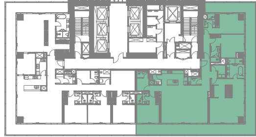
29TH TO 33RD FLOOR
