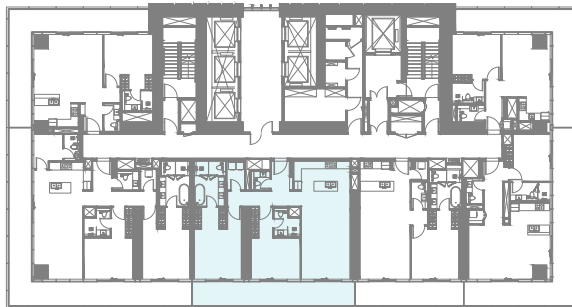
1ST TO 9TH, 14TH TO 21ST & 23RD TO 27TH FLOOR
